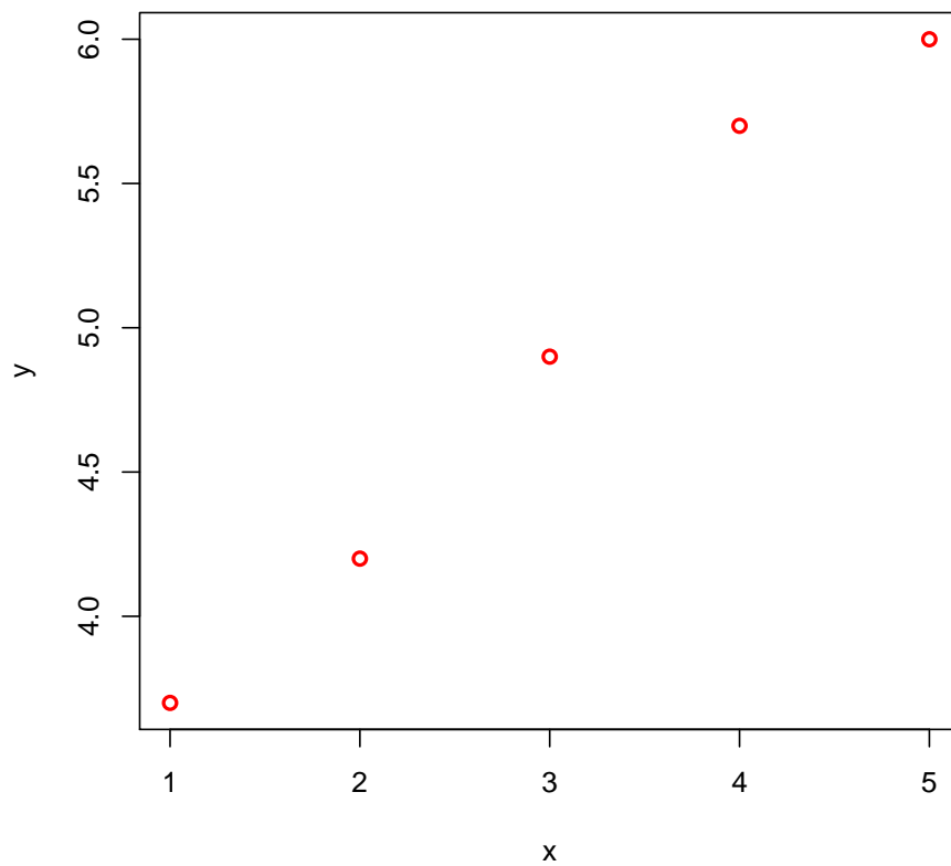
Figure 2.1: Regression
