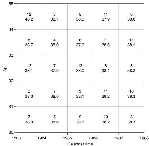
Tabulation in the Lexis diagram (Lexis-tab)
