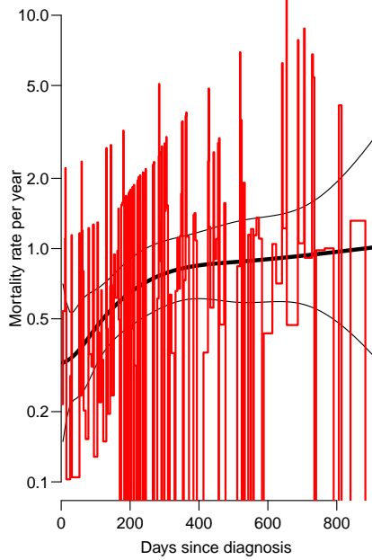
Who needs the Cox-model anyway? (KMCoz)
