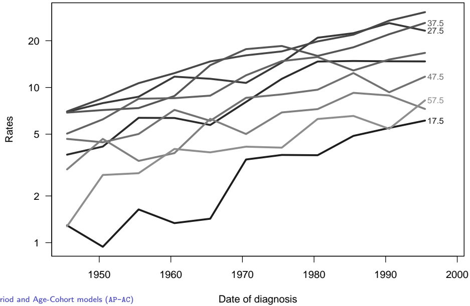
Age-Period and Age-Cohort models (AP-AC)
