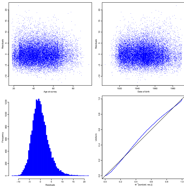
Continuous outcomes (cont)
